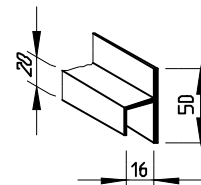
Top Cap Profile
